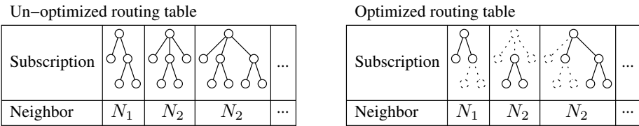
Fig. 3. Event routing table before (left) and after (right) applying subscription pruning
