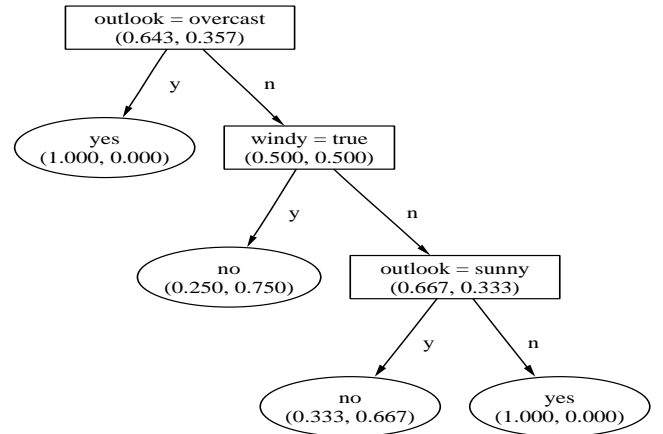
Figure 1: A sample decision tree for the weather dataset.
