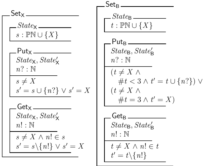
Fig. 7. \text{Set}_A \sqsubseteq_{sub}^{\{X\}} \text{Set}_X and \text{Set}_X \sqsubseteq \text{Set}_B
