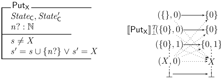
Fig. 6. \text{Put}_A \sqsubseteq_{sub}^{\{X\}} \text{Put}_X
