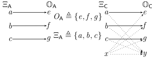
Fig. 3. A \sqsubseteq_{sub}^{AC} C
