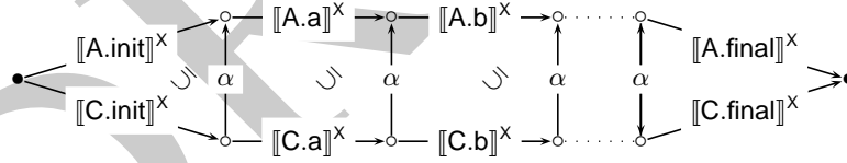
Fig. 2. Backward simulation
