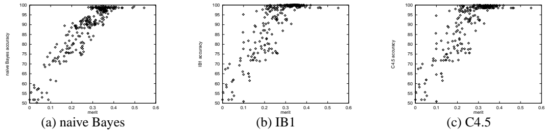
Figure E.1: Mushroom (mu).
