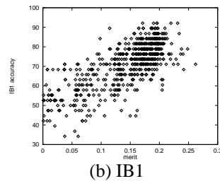
Figure E.8: Dna-promoter (dna).
