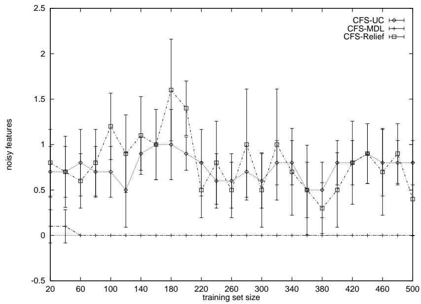
Figure B.4: Number of noisy attributes selected on concept A3 by CFS-UC, CFS-MDL, and CFS-Relief as a function of training set size.
