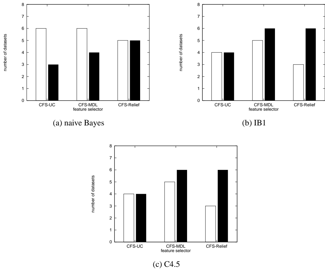
Figure 6.20: Number of natural domains for which CFS improved accuracy (left) and degraded accuracy (right) for naive Bayes (a), IB1 (b), and C4.5 (c).
