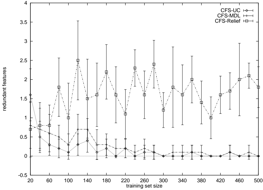
Figure 6.11: Number of redundant attributes selected on concept A1 (with added redundant features) by CFS-UC, CFS-MDL, and CFS-Relief as a function of training set size.
