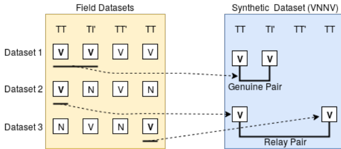
Fig. 5. Synthetic Data Generation (VNNV)
