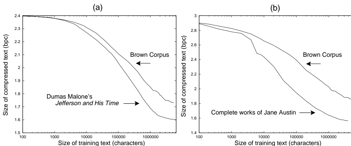
Figure 1: How training text improves compression for PPM (a) for the last chapter of Dumas Malone's Jefferson the Virginian (b) for the last chapter of Jane Austin's Emma
