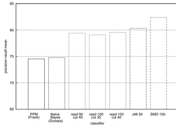
Fig. 8. Comparing 7 classifiers' precision-recall mean macroaverage over the 10 largest Reuters categories.
