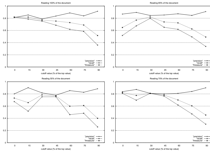
Fig. 7. Effects of pruning dictionaries and reading only initial parts of documents.
