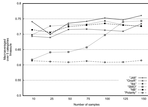
Fig. 6. Macroaverages for 6 classifiers plotted per number of attributes.
