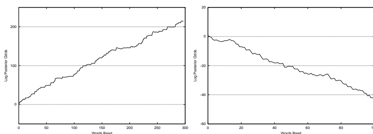
Fig. 1. Illustration of document profiles, the left hand side one is about the topic while the right hand side one is not.
